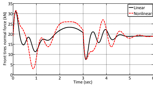
Figure 19. Front tire normal force
